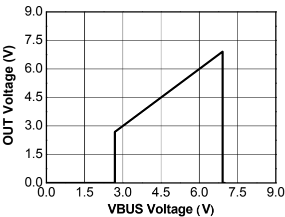
Figure 11. OUT Voltage vs VBUS Voltage
