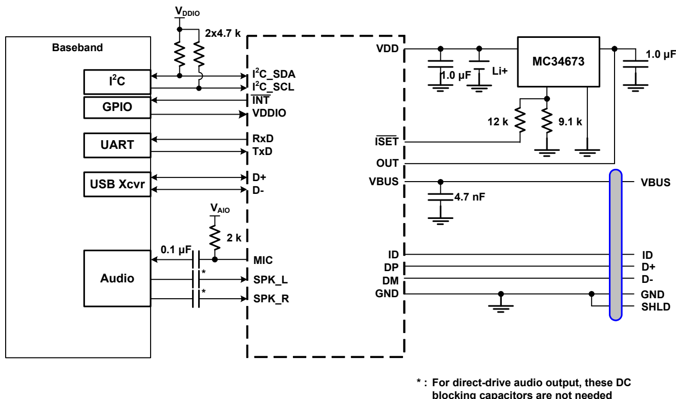
Figure 27. Interface Circuit in a Cell Phone System
